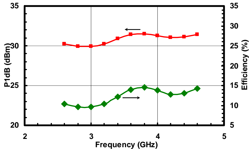
Figure 2: P_{1dB} and Efficiency ( V_{dd} = 12V ) versus Frequency
