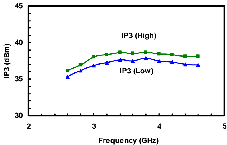
Figure 4: Third order inter-modulation intercept versus Frequency
