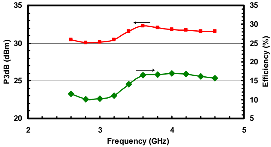
Figure 3: P_{3dB} and Efficiency ( V_{dd} = 12V ) versus Frequency
