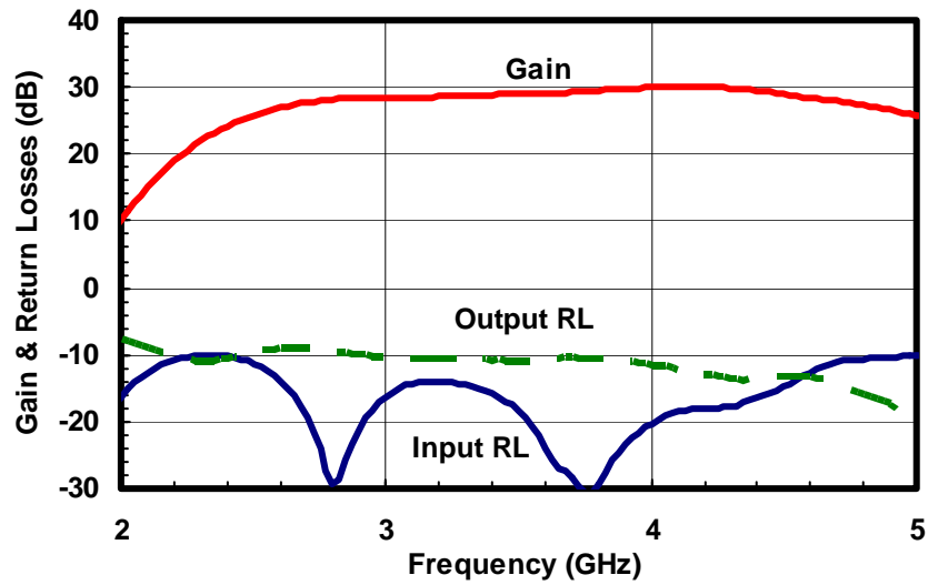
Figure 1: Gain and return loss as a function of frequency. ( V_{dd} = +12V , I_{dq}=0.9A , T_a=25^{\circ}C )
